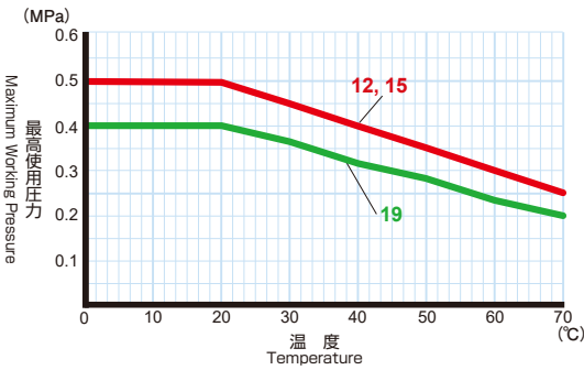
〔E-KYC の使用温度と最高使用圧力の関係図〕 E-KYC: Relationship between Working Temperature and Maximum Working Pressure
