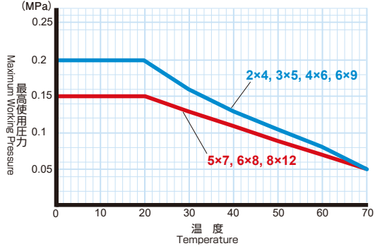
〔E-KYT の使用温度と最高使用圧力の関係図〕 E-KYT: Relationship between Working Temperature and Maximum Working Pressure
