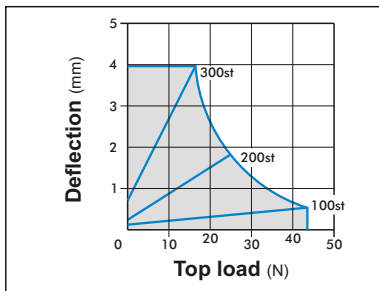
MCGA-23... φ 20
