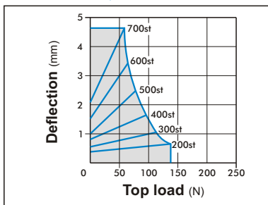
MCGA-63... φ 50
