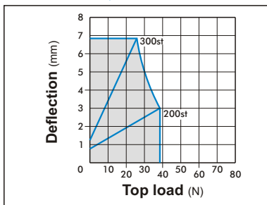
MCGA-63... φ 20
