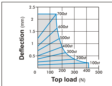
MCGA-23... φ 50
