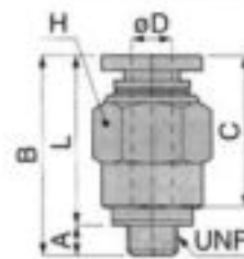
Appearance Dimension for Unified thread
