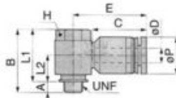
Appearance Dimension for Unified thread
