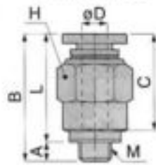
Appearance Dimension for Metric thread
