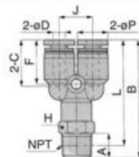
Appearance Dimension for Pipe thread general purpose (NPT)
