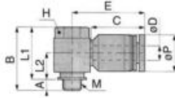
Appearance Dimension for Metric thread
